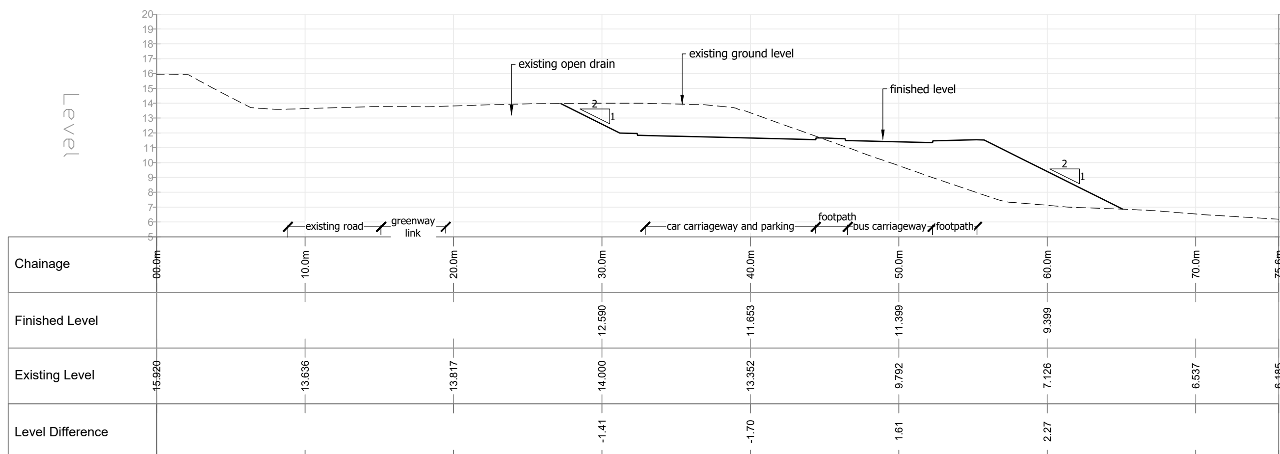
BUS PARK SECTION 02
