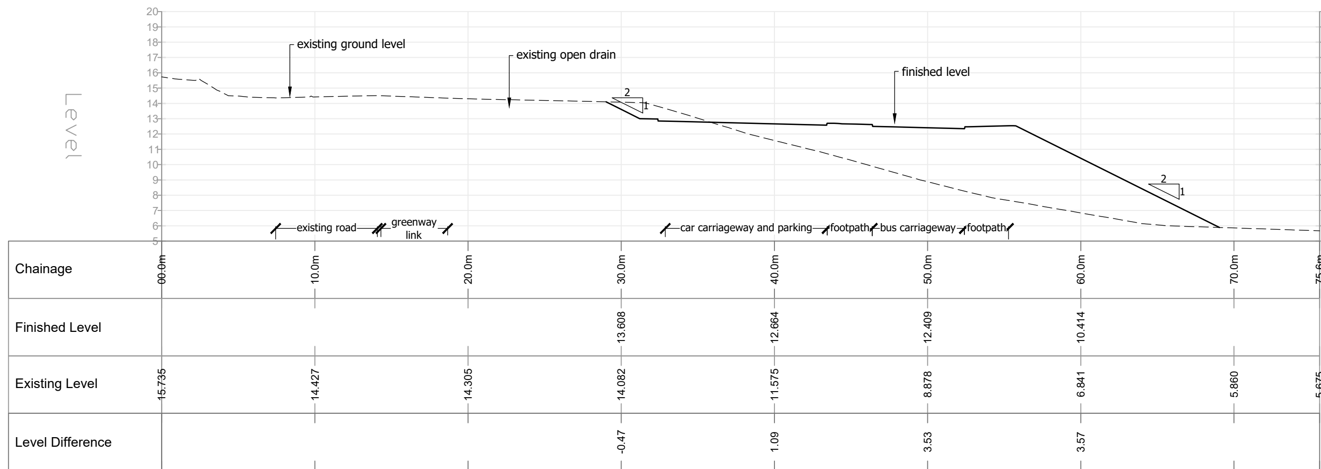
BUS PARK SECTION 01
